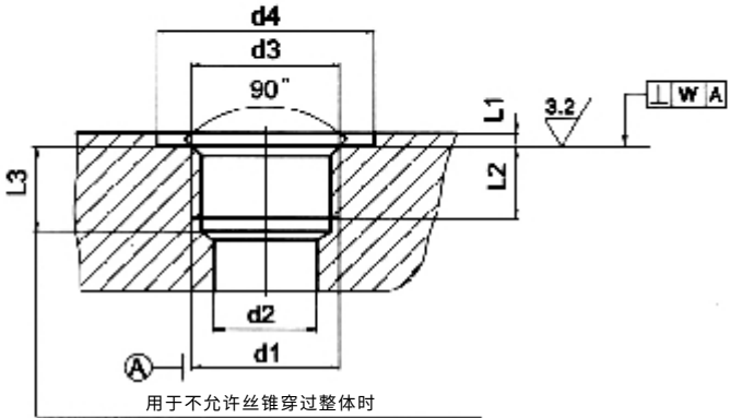
This dimension only applies when tap drill cannot pass through tire boss ISO 9974-1 油口 Port
