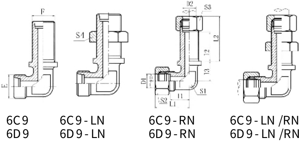
90° 弯曲过板接头 90° ELBOW BULKHEAD FITTINGS
